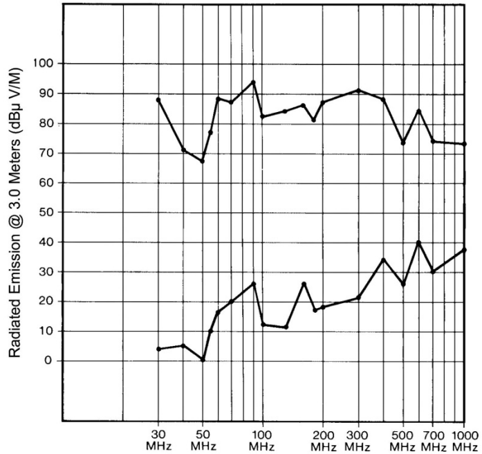
Radiated Emission Comparison Unshielded vs. CW Shielded D-Subminiatures Assemblies
