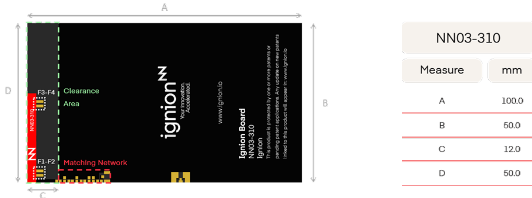
Figure 2 – PCB layout from the Antenna Intelligence Cloud™.
