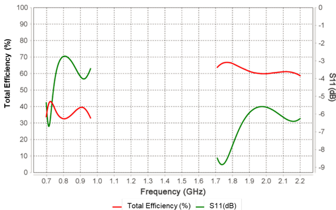
Figure 4 – Reflection Coefficient (dB) and Total Efficiency (%) from the Antenna Intelligence Cloud™.
