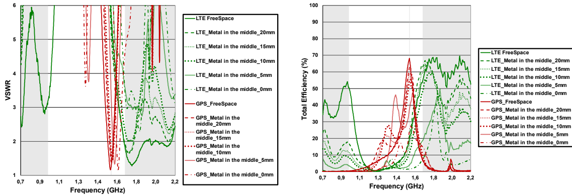
Figure 28 – VSWR & total efficiency for the different bands covered by the L size board from Figure 10 and placed in close proximity to metal.
