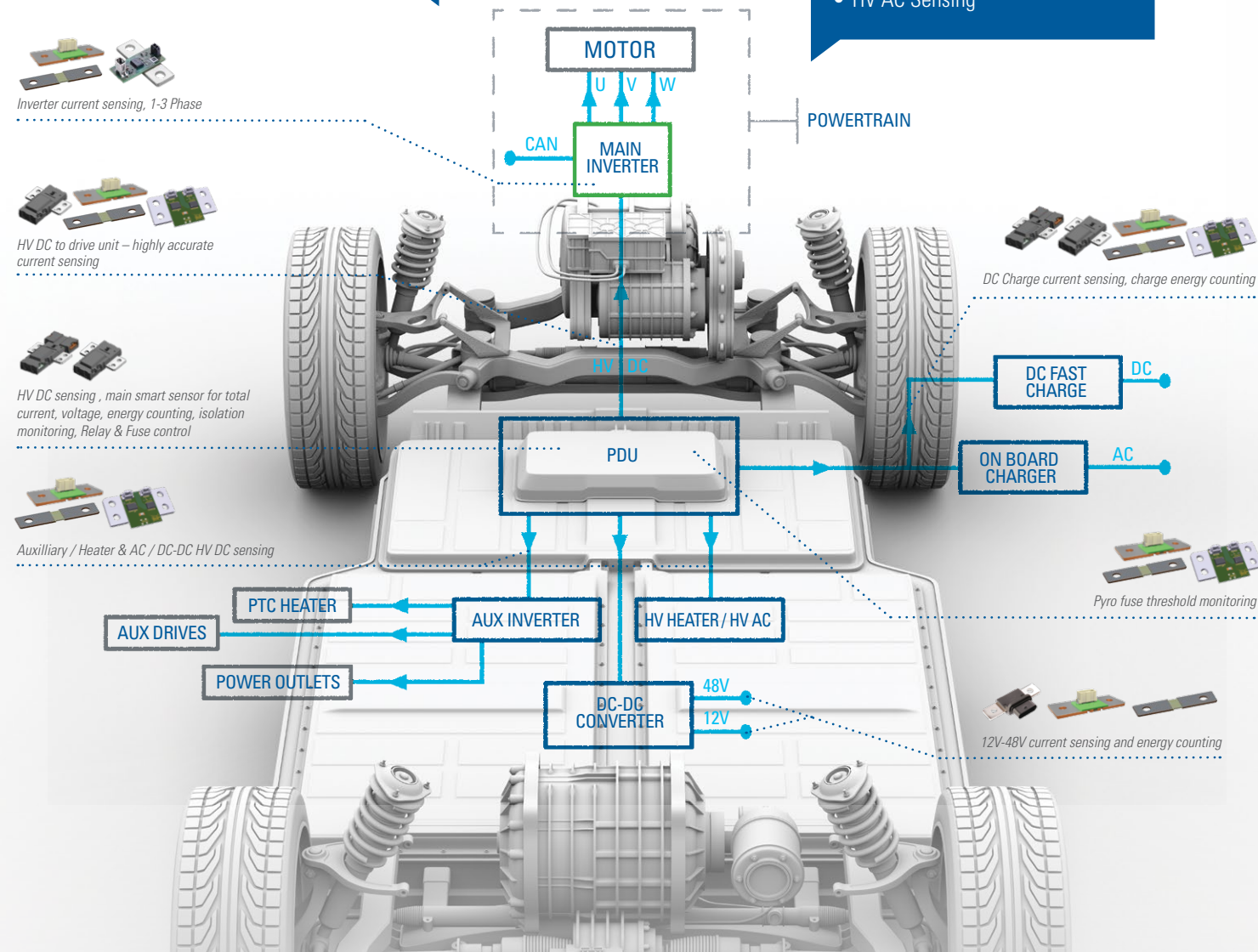
Auxiliary Power Outlets • HV DC sensing • 12V to 48V DC • HV AC Sensing
