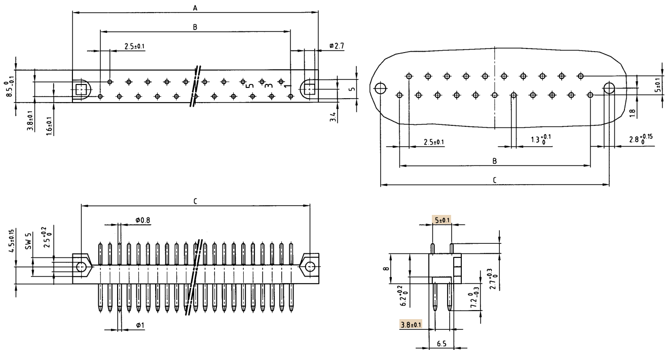
PCB-hole pattern
