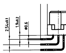
Solder pin angled
