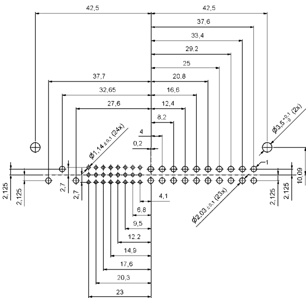
PCB-hole pattern
