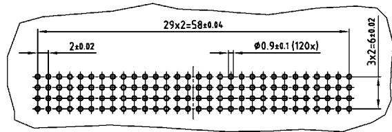
PCB-hole pattern
