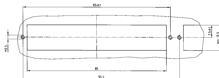
Panel cutout
