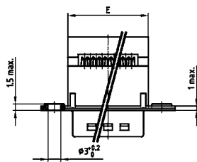
Strain relief
