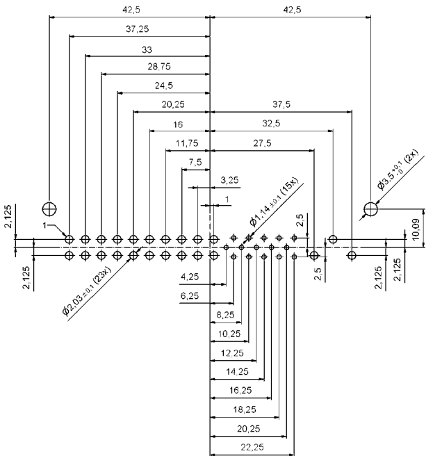
PCB-hole pattern
