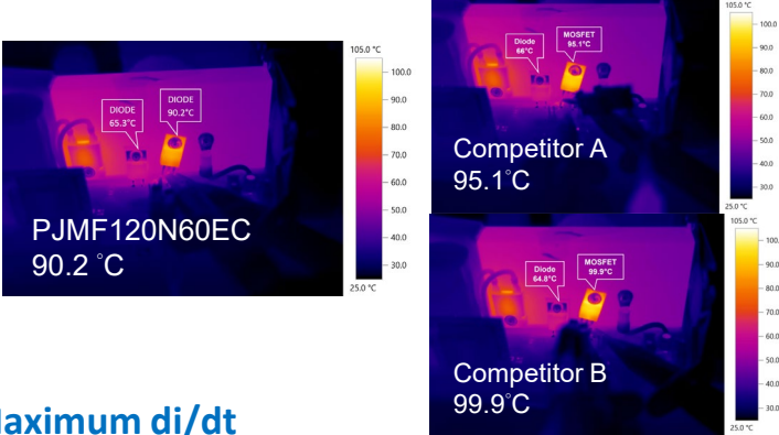
Junction Temperature @ Full Load Operation
