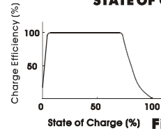
Figure 23. CHARGING EFFICIENCY VS STATE OF CHARGE
