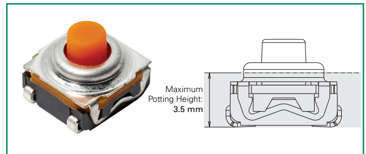
Figure 3: KSC PF Series Tactile Switch (Potting-Friendly) With Extended Cage
