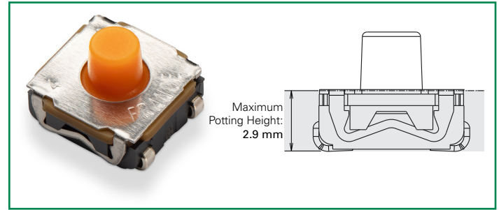
Figure 2: KSC4 Series Tactile Switch Standard Version With Flat Cage
